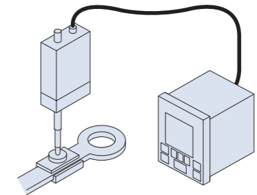
Measurement of crimp height Measures the calking height of crimp terminal.
